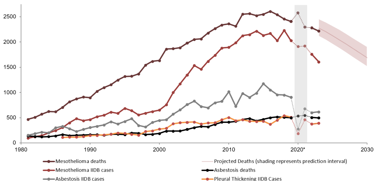
Figure 1: Mesothelioma, asbestosis, and pleural thickening: time trends in annual deaths and Industrial Injuries Benefit Disablement (IIBD) cases
