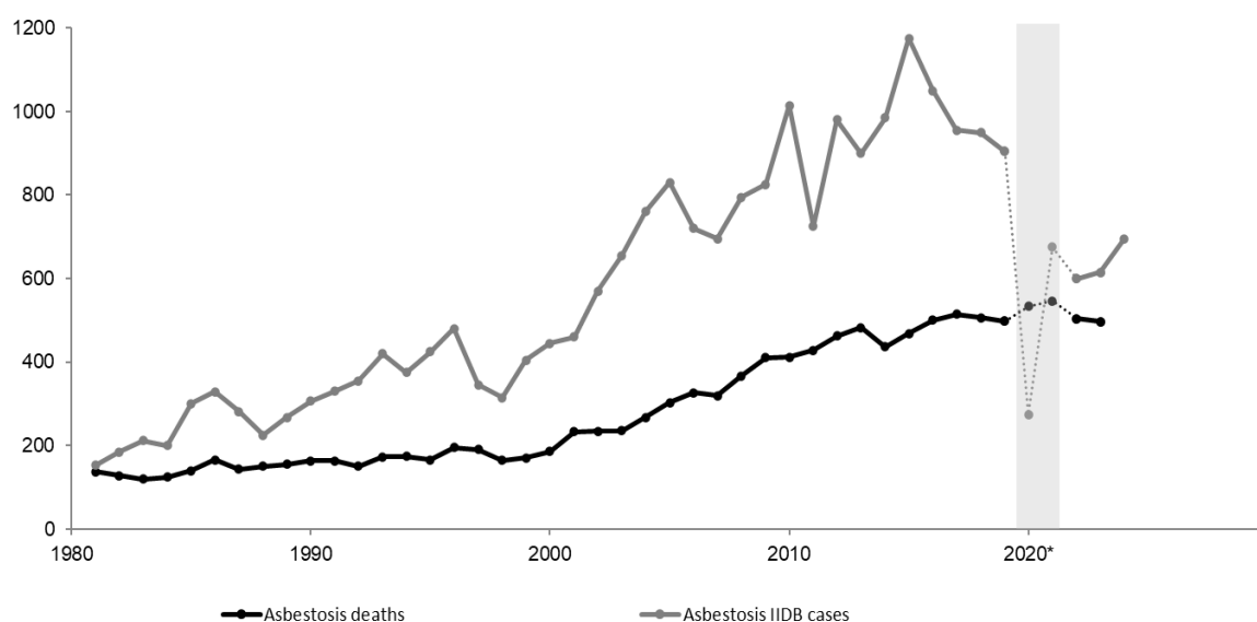
Figure 2: Annual deaths where death certificates mentioned asbestosis but not mesothelioma 1978-2023, and IIDB cases 1978-2024
