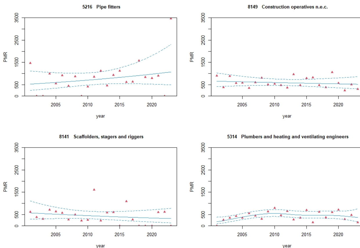
Figure A3.4a: Asbestosis PMRs by SOC unit group, males, 2001-2023
