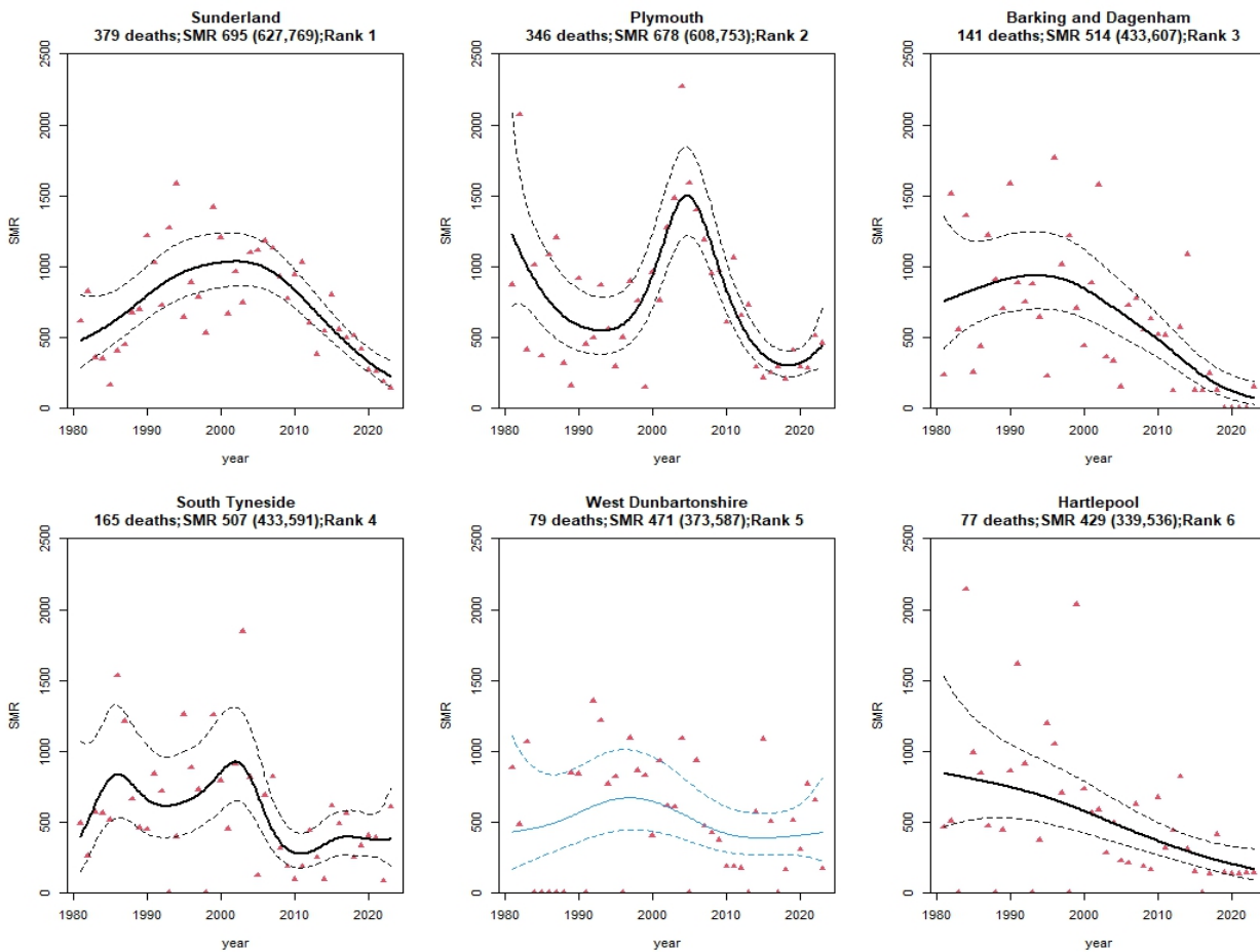
Figure A1.4 – Annual asbestosis SMRs for males for the top six U/LA areas, 1981-2023
